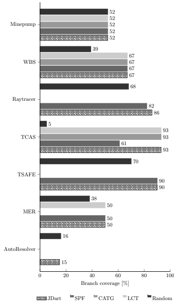
Fig. 8: Branch coverage.
